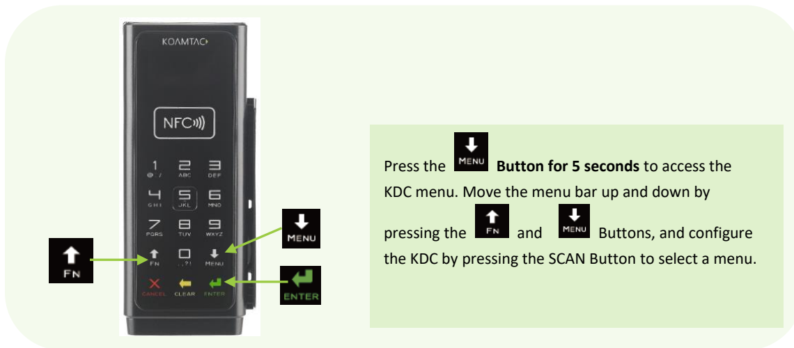
Figure 10 - Location and use of buttons on a keypad (KDC500)
