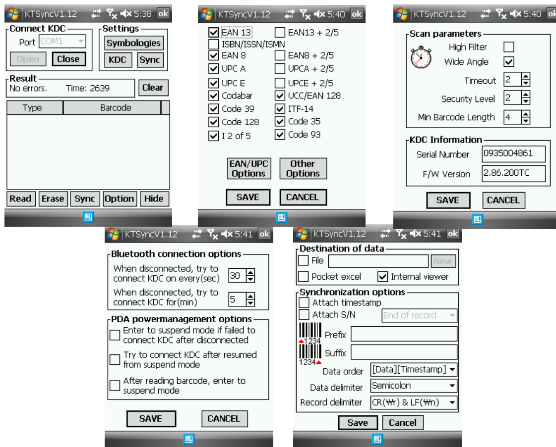
Figure 28 - Mobile pKTSync
