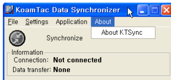
Figure 20 - About Menu
