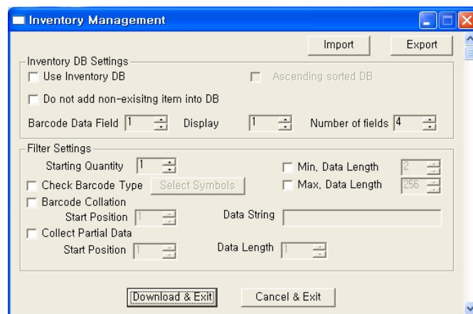
Figure 41 – Inventory Application
