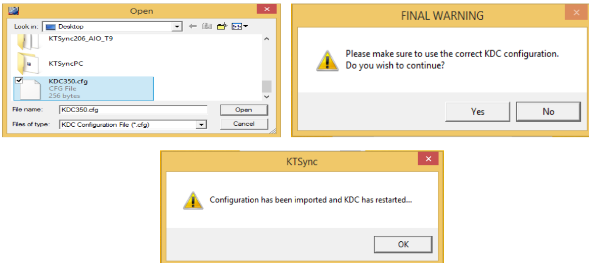
Figure 23 – Configuration
