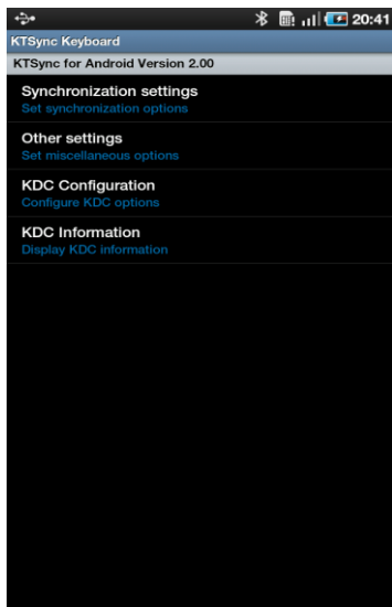
Figure 29 - Android aKTSync
