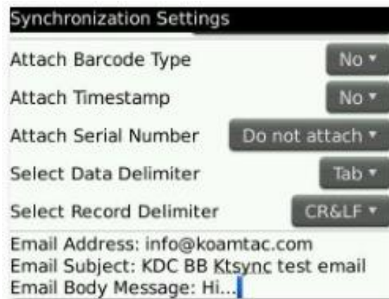
Figure 31 - Blackberry bKTSync
